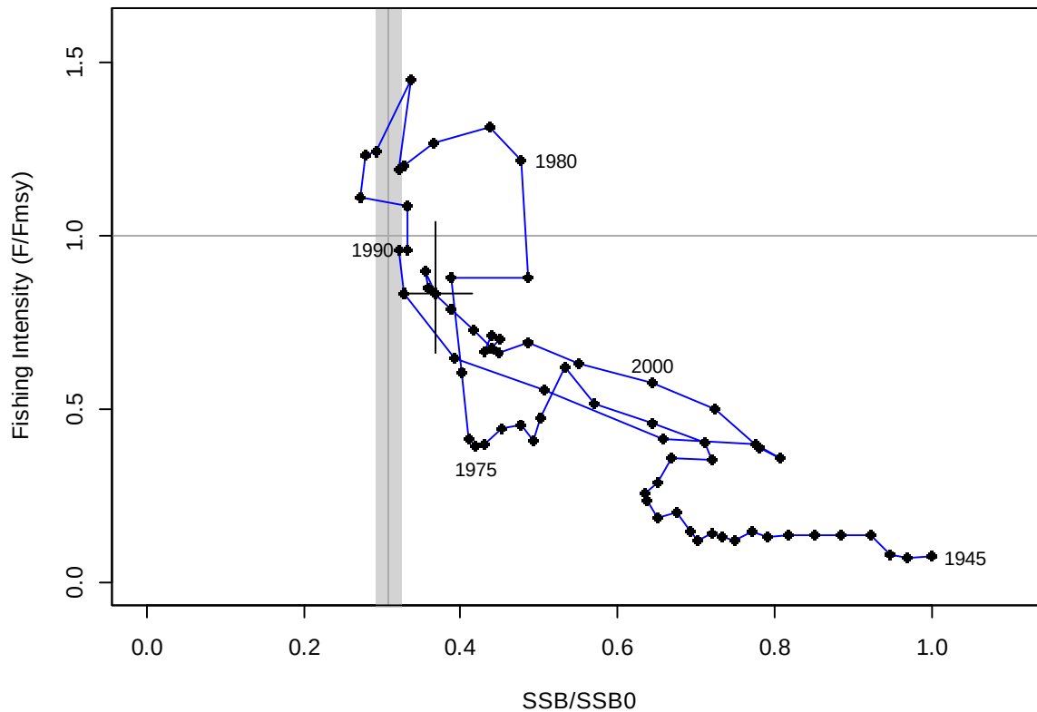
Figure 12: Phase plot that summarises the SSB history of the CRA 2 stock. The x-axis is spawning stock biomass SSB in each year as a proportion of the unfished spawning stock, SSB_0 . The y-axis is fishing intensity in each year as a proportion of the fishing intensity ( F_{msy} ) that would have given MSY under the fishing patterns in that year. Each point on the figure shows the median of the posterior distributions of biomass ratio and fishing intensity ratio for one year. The vertical line in the figure is the median (line) and 90% interval (shading) of the posterior distribution of SSB_{msy} ; this ratio was calculated using the fishing pattern in 2012. The horizontal line in the figure is drawn at 1, the fishing intensity associated with F_{msy} . The bars at the final year of the plot (2012) show the 90% intervals of the posterior distributions of biomass ratio and fishing intensity ratio.
