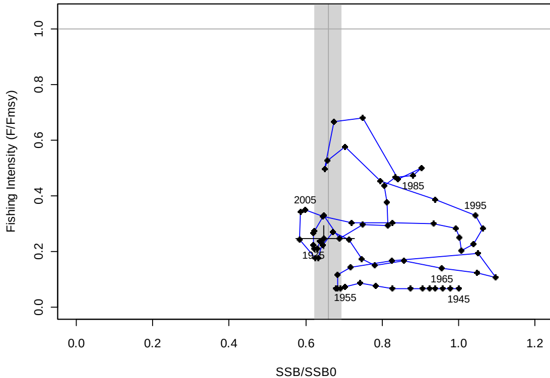
Figure 15: Phase plot that summarises the SSB history of the CRA 4 stock. The x-axis is spawning stock biomass SSB in year y as a proportion of the unfished spawning stock, SSB_0 . SSB_0 is constant for all years of a run, but varies through the 1000 runs. The y-axis is fishing intensity in year y as a proportion of the fishing intensity ( F_{msy} ) that would have given MSY under the fishing patterns in year y ; fishing patterns include MLS, selectivity, the seasonal catch split and the balance between SL and NSL catches. The vertical line in the figure is the median (line) and 90% interval (shading) of the posterior distribution of SSB_{msy} (the spawning stock biomass associated with MSY) as a proportion of SSB_0 ; this ratio was calculated using the fishing pattern in 2010. The horizontal line in the figure is drawn at 1, the fishing intensity associated with F_{msy} . The bars at the final year of the plot show the 90% intervals of the posterior distributions of biomass ratio and fishing intensity ratio.
