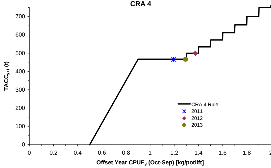
Figure 6: The CRA 4 management procedure, showing the TACC in year y+1 as a function of offset year CPUE in year y , and showing the TACCs resulting from the rule evaluations performed in 2011, 2012 and 2013 for the 2012–13, 2013–14 and 2014–15 fishing years.
