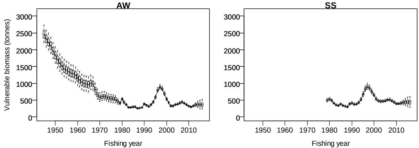
Figure 11: Posterior distributions of the CRA 2 base case McMC vulnerable biomass trajectory by season. Before 1979 there was a single time step, shown in AW. For each year the box spans the 25th and 75th quantiles and the whiskers span the 5th and 95th quantiles.
